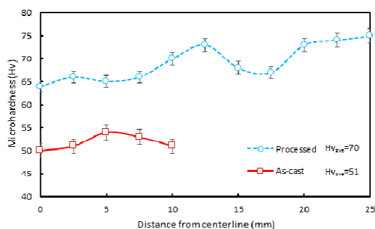
Fig. 5. Microhardness variations along with samples diameter
