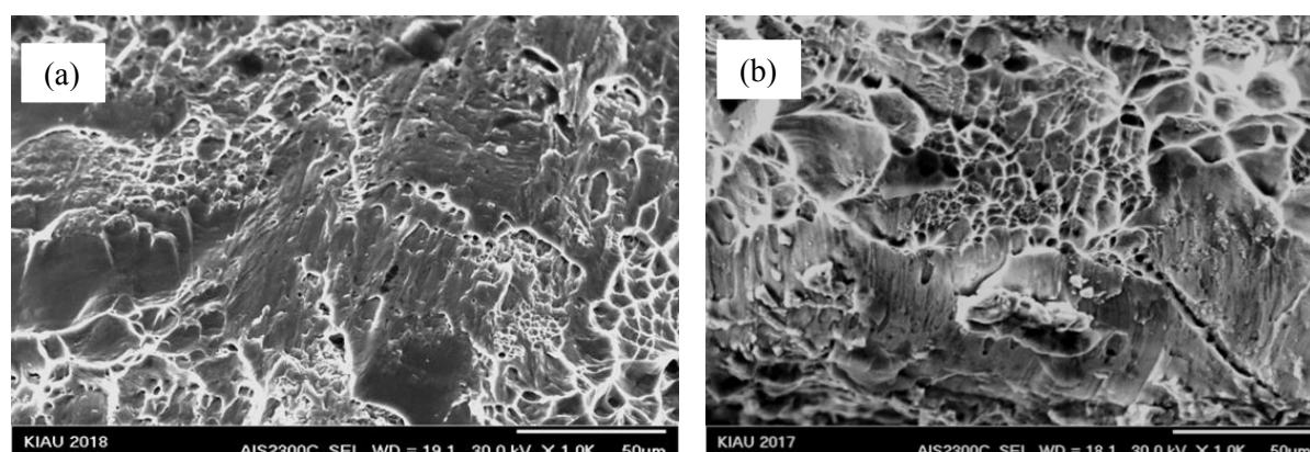
Fig. 5. SEM micrographs of the fracture surfaces in a) 400°C annealed and b) 500°C annealed alloys.
