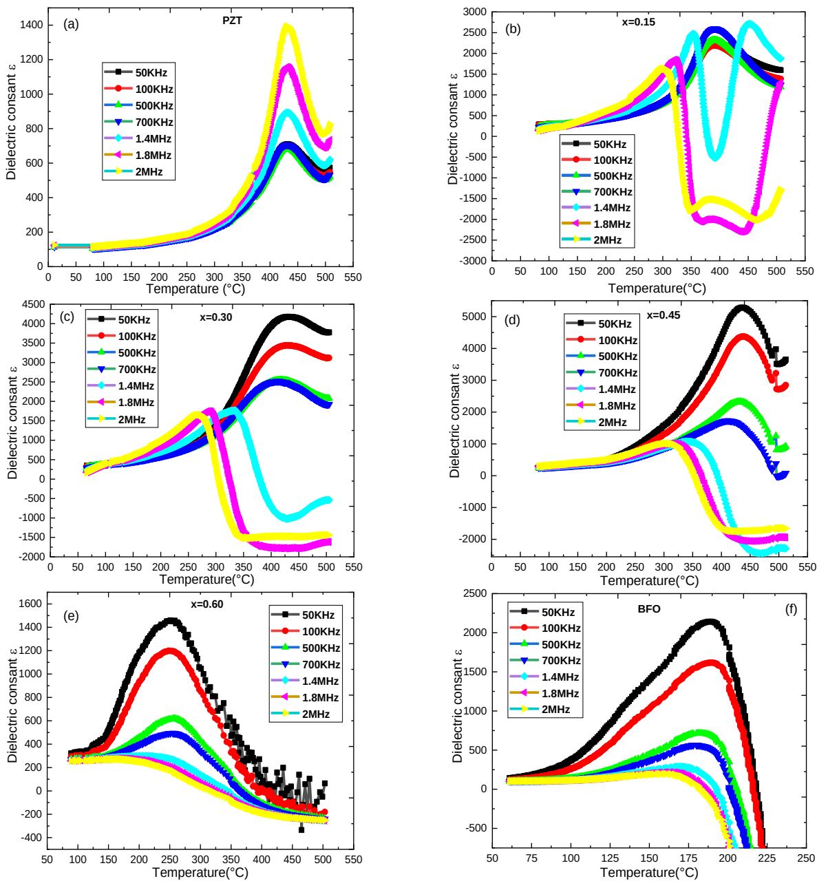
Fig. 8. Evolution of dielectric permittivity of sintered (1-x)PZT-xBFO composites at 950°C/2 h as a function of temperature at different frequencies
