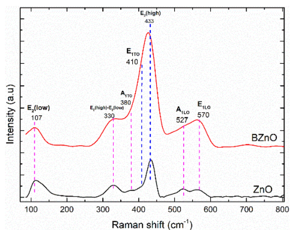
Fig. 5. Raman spectra of ZnO and BZnO microrods
