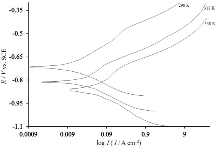
Fig. 4. Anodic and cathodic polarization curves for mild steel in alkaline 3% NaCl (pH=10) with 7×10 -5 M of inhibitor at different temperatures: 298 K, 318 K and 338 K.
