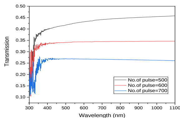
Fig. 6. Transmittance of the \text{TiO}_2/\text{MgO} nanocomposite at variable of laser shots.
